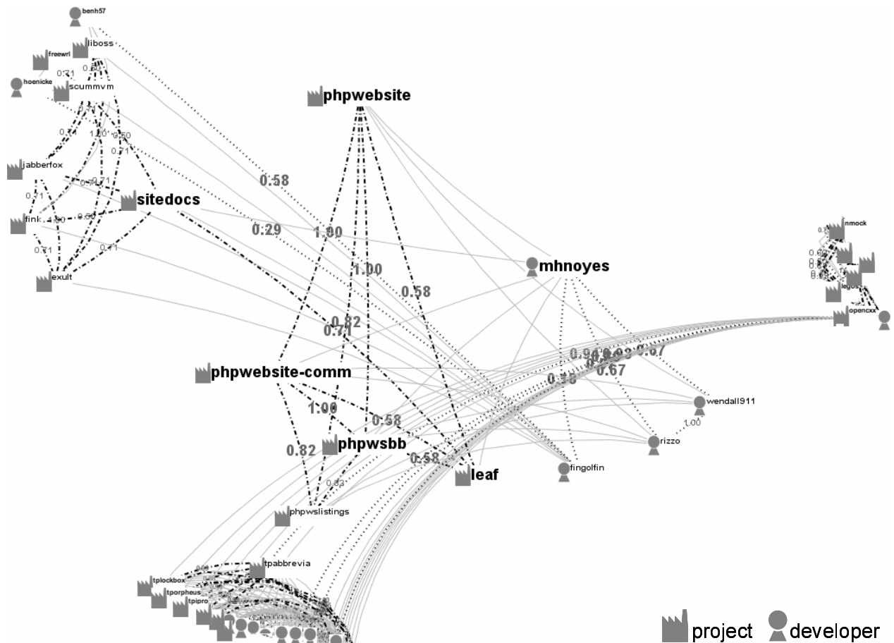
Figure 1: Developer-project networks (numbers in-between edges are the degree of similarity between nodes)
