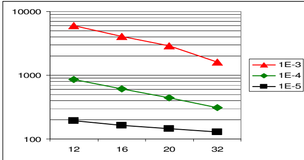
Figure 2. Impact of the cepstra series cardinality over the number of pairs deemed similar (logarithmic).
