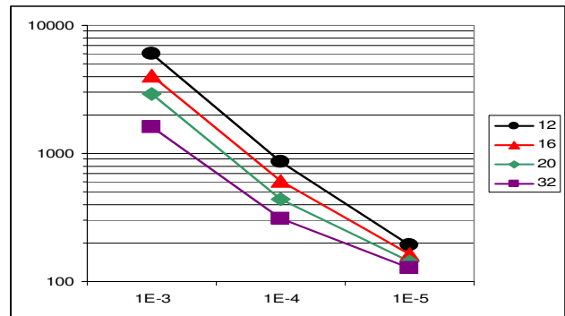
Figure 1. Impact of the threshold over the number of pairs deemed similar (logarithmic).
